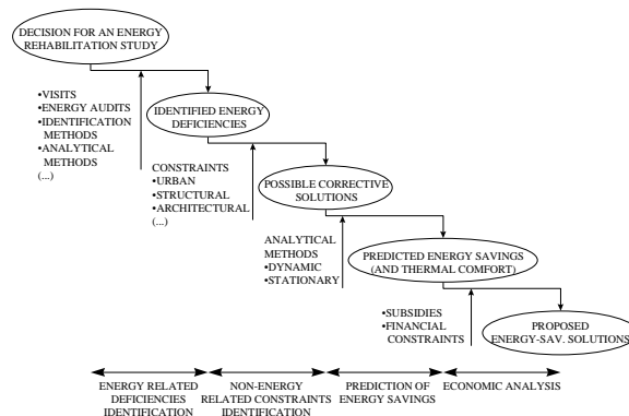
Figure 1: Different steps in the diagnosis stage of an energy rehabilitation study.
