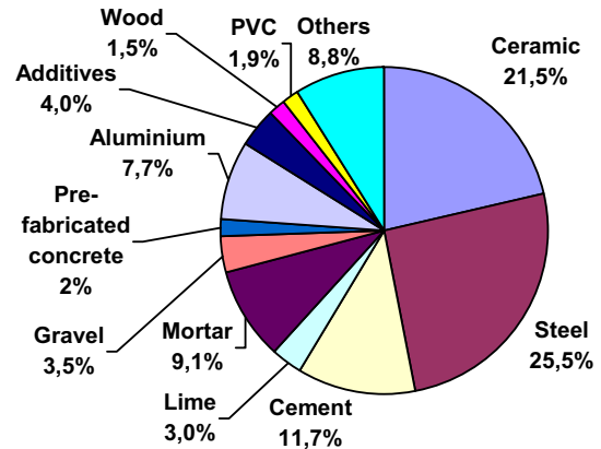
Fig. 1. Contribution of primary energy demand for the manufacture of the materials needed in the construction of 1 m 2 (gross floor area) [12].
