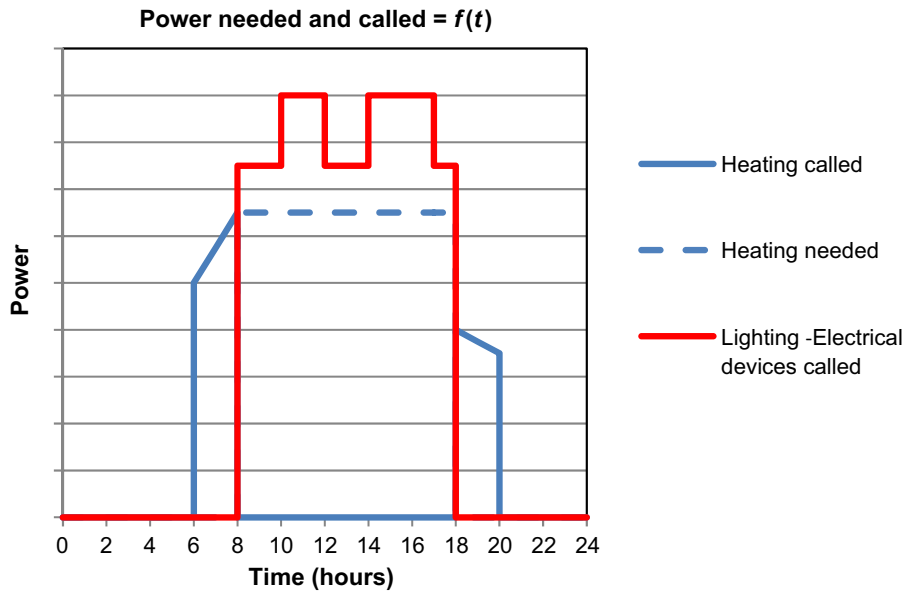
Figure 8 Example of interoperability between the electrical loads and the heating system.
