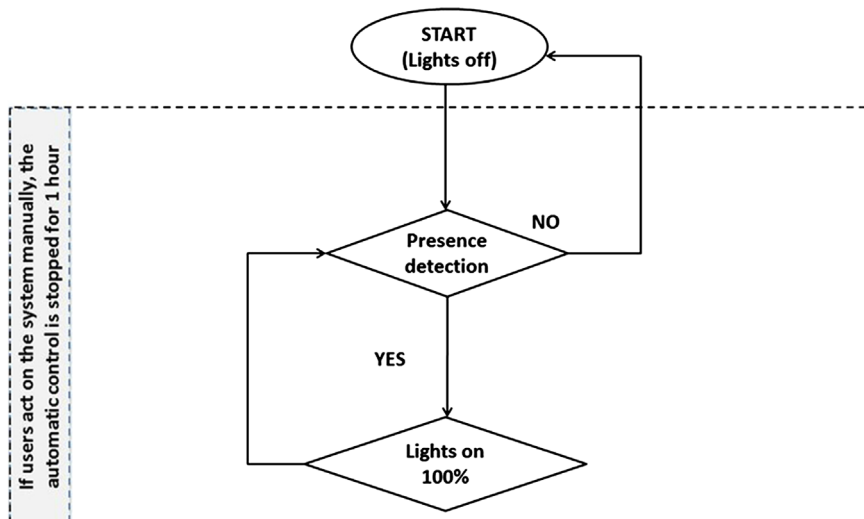
Figure 3 Control logic in case of occupancy control in open plan offices.
