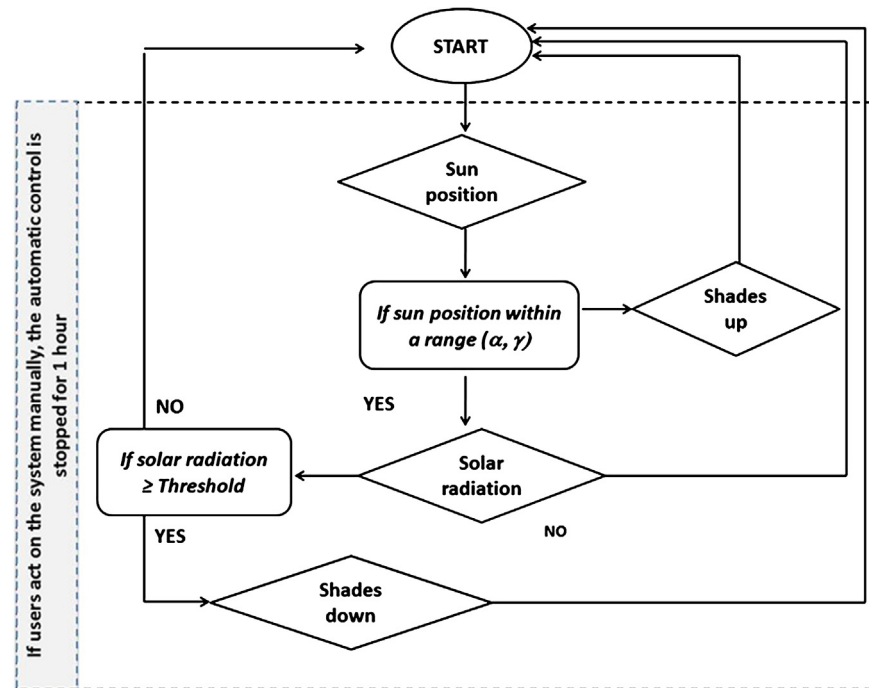
Figure 5 Control logics in case of shading devices.
