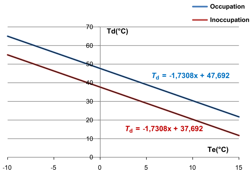
Figure 14 Hot water calculation law used.
