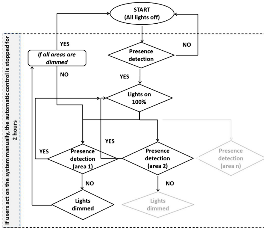
Figure 4 Control logic in case of occupancy control in classrooms.
