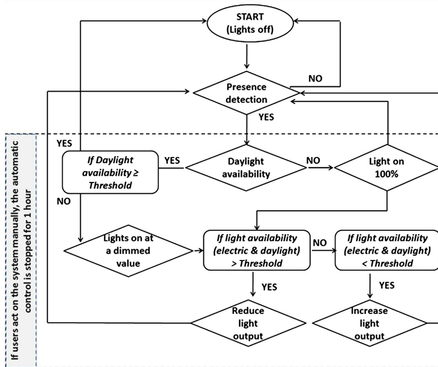
Figure 2 Control logic in case of both daylight harvesting and occupancy control.
