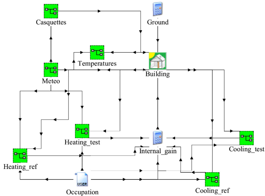
Figure 12 Global TRNSYS simulation model.
