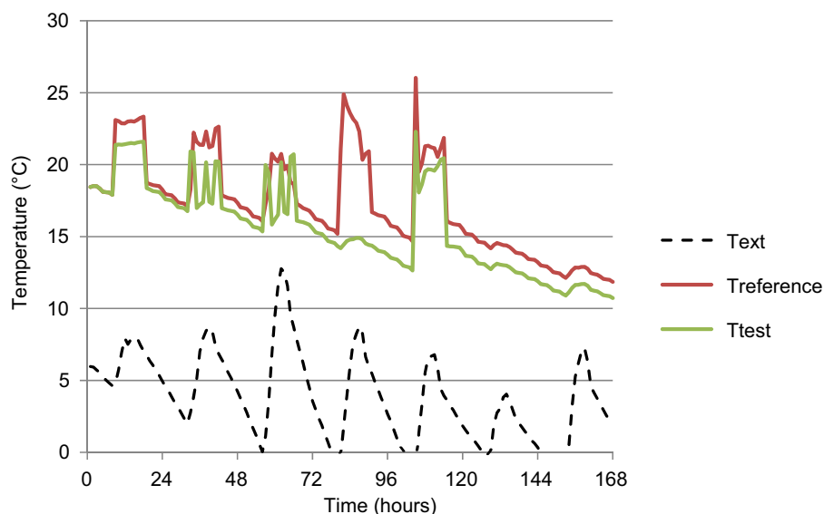
Figure 15 Indoor temperatures results of the simulation.
