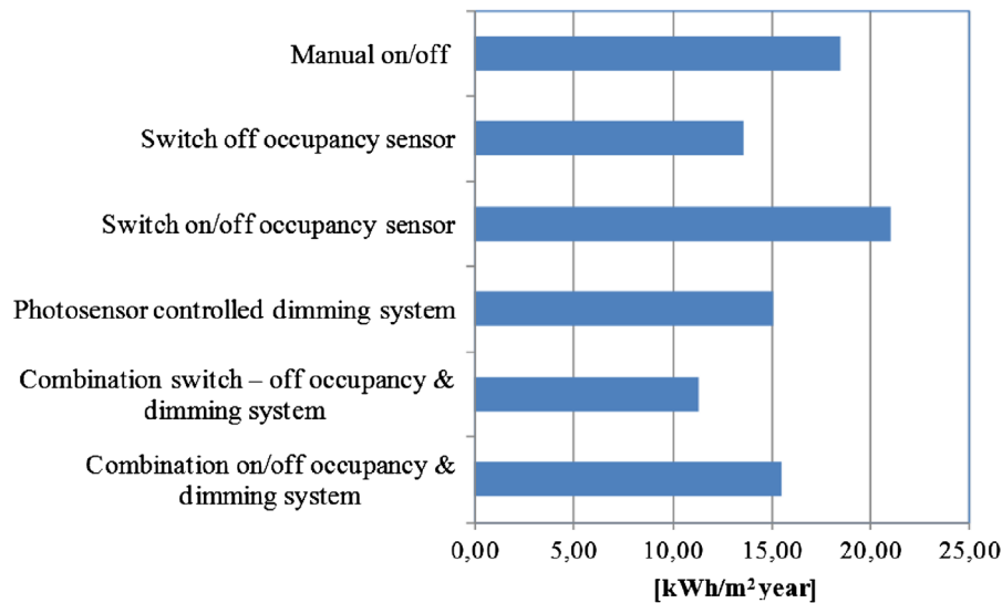
Figure 11 Energy demand for different control strategies.
