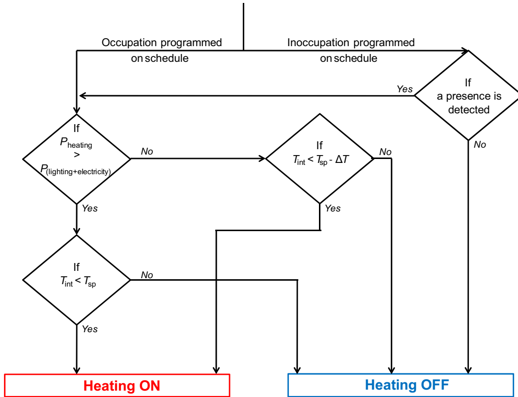
Figure 7 Algorithm for heating strategy.
