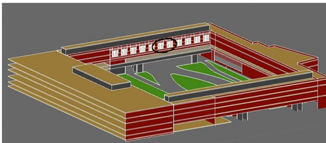
Figure 10 3D model of the building around the simulated rooms.
