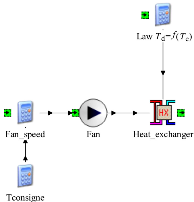
Figure 13 TRNSYS simulation model to simulate fan coils.
