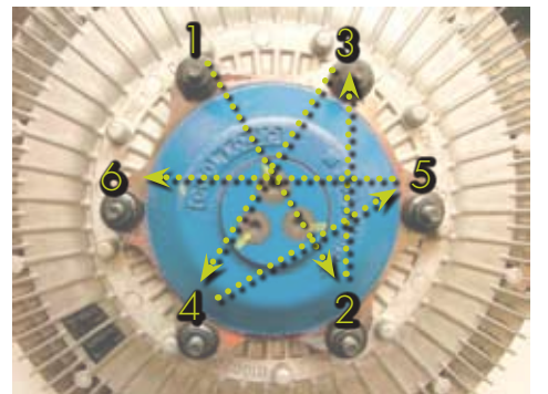
Figure 3 Torque sequence
