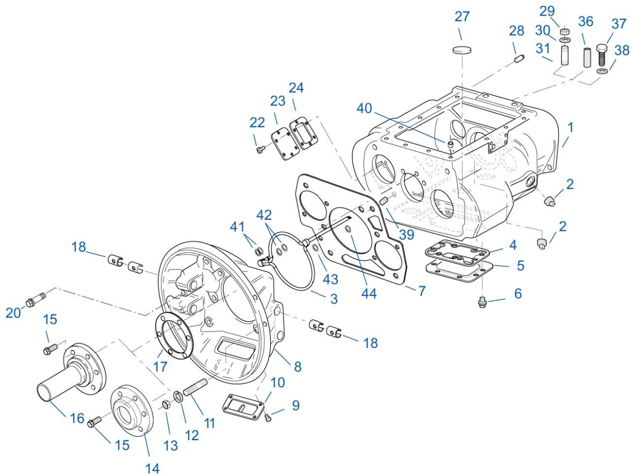
10319-11-99 Alum Hsg
