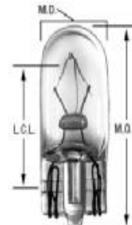
LMP194 T3-1/4 BOMBILLO LAGRIMA 12V
