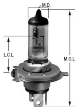
LMP9003 BOMBILLO HALOG. T-4- 5/8 12V
